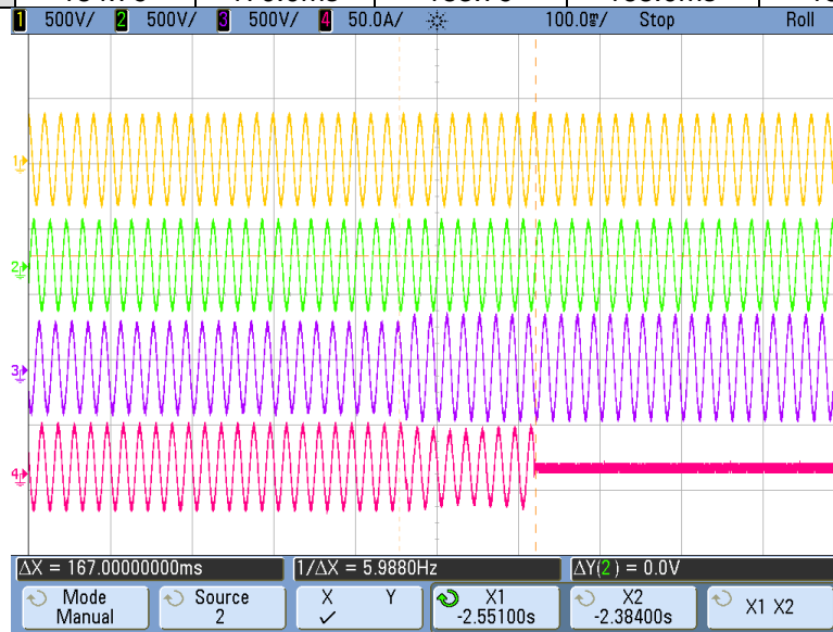
Overvoltage Protection
