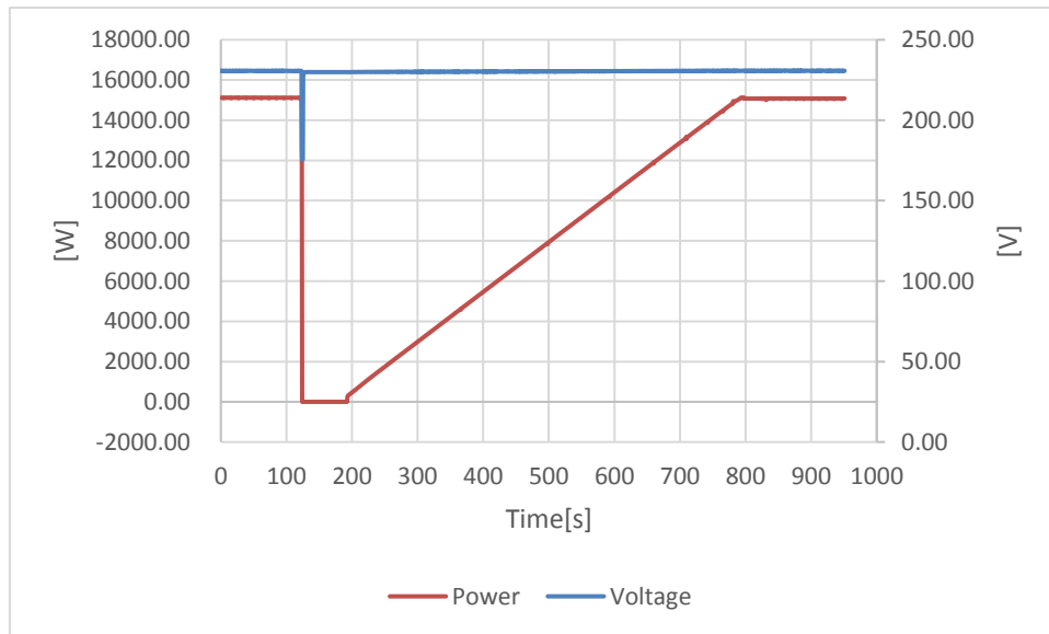
After 2s of 77% U n
