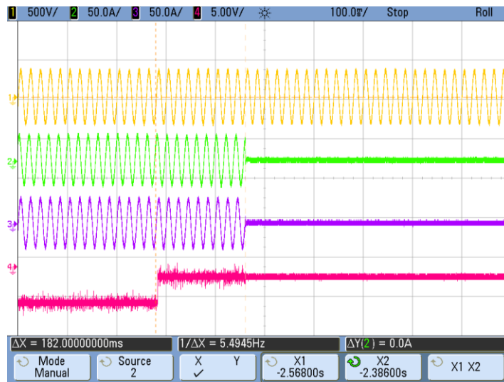
Feed-in current at 100%P
