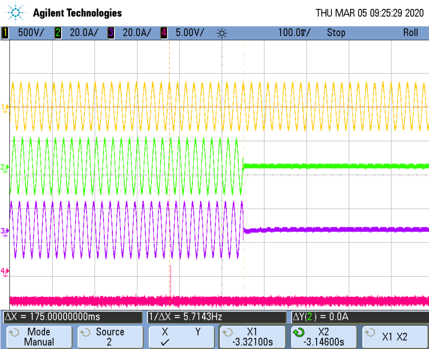
Frequency increase
