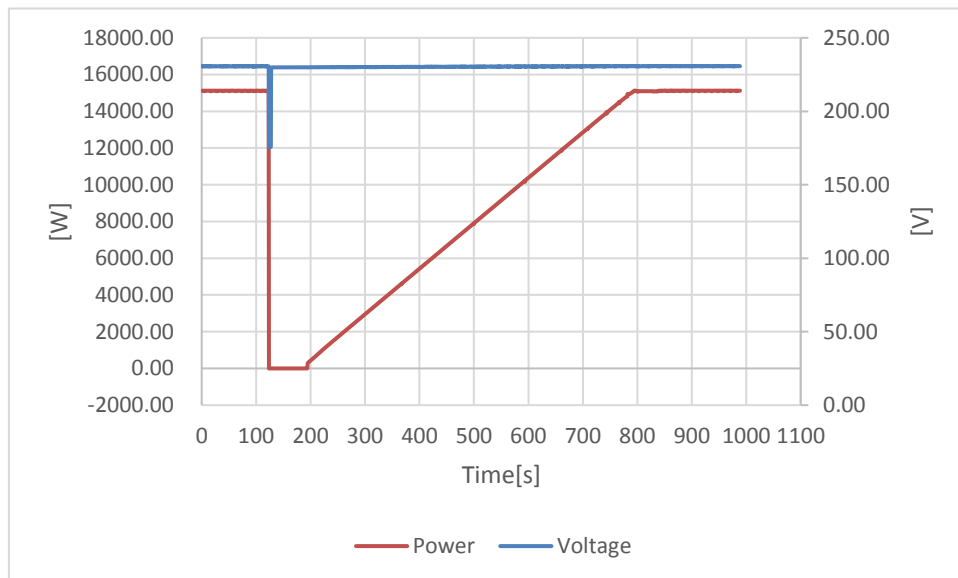
After 4s of 77% U n
